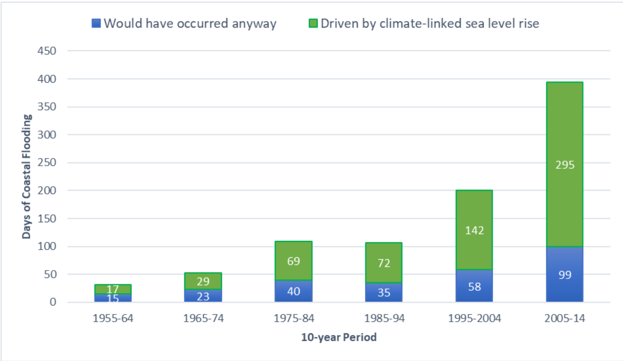
Figure 20. Coastal flood days in Prince George's County Area. Data pulled from a U.S. Naval Academy water level station, 22 miles from Prince George's County. ( Climate Central Risk Finder ).
