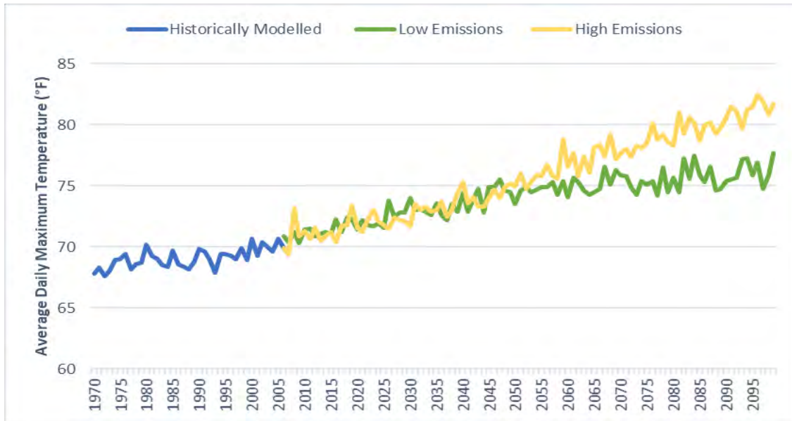
Figure 2. Projected increase of average daily maximum temperature in Prince George’s County (U.S. Climate Resilience Toolkit Climate Explorer).
